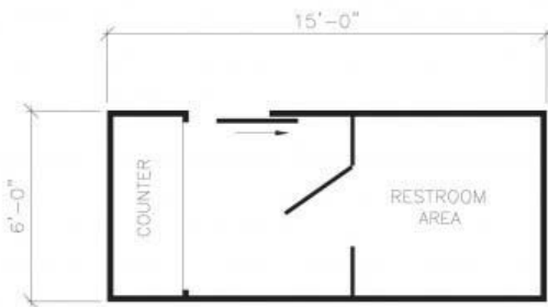
Guard Booth w/Restroom Interior Restroom Entry Door
