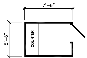
Rear Swing Door
