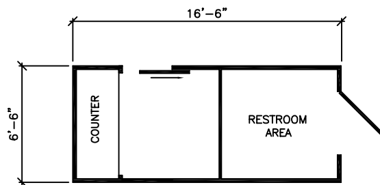
Guard Booth with Restroom Exterior Restroom Entry Door
