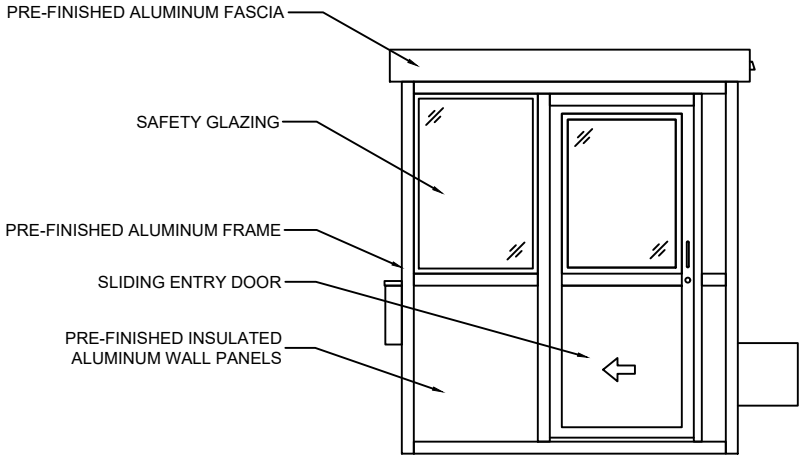
Elevation "A"
