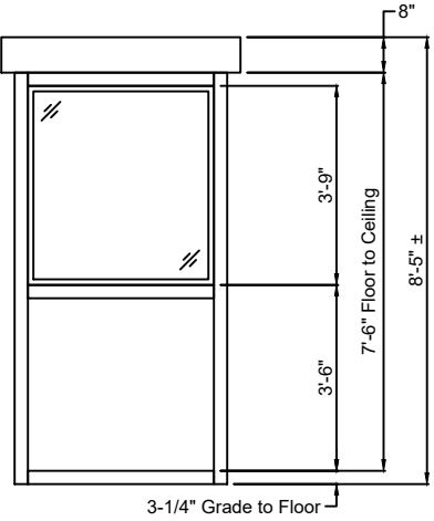
Elevation "B"
